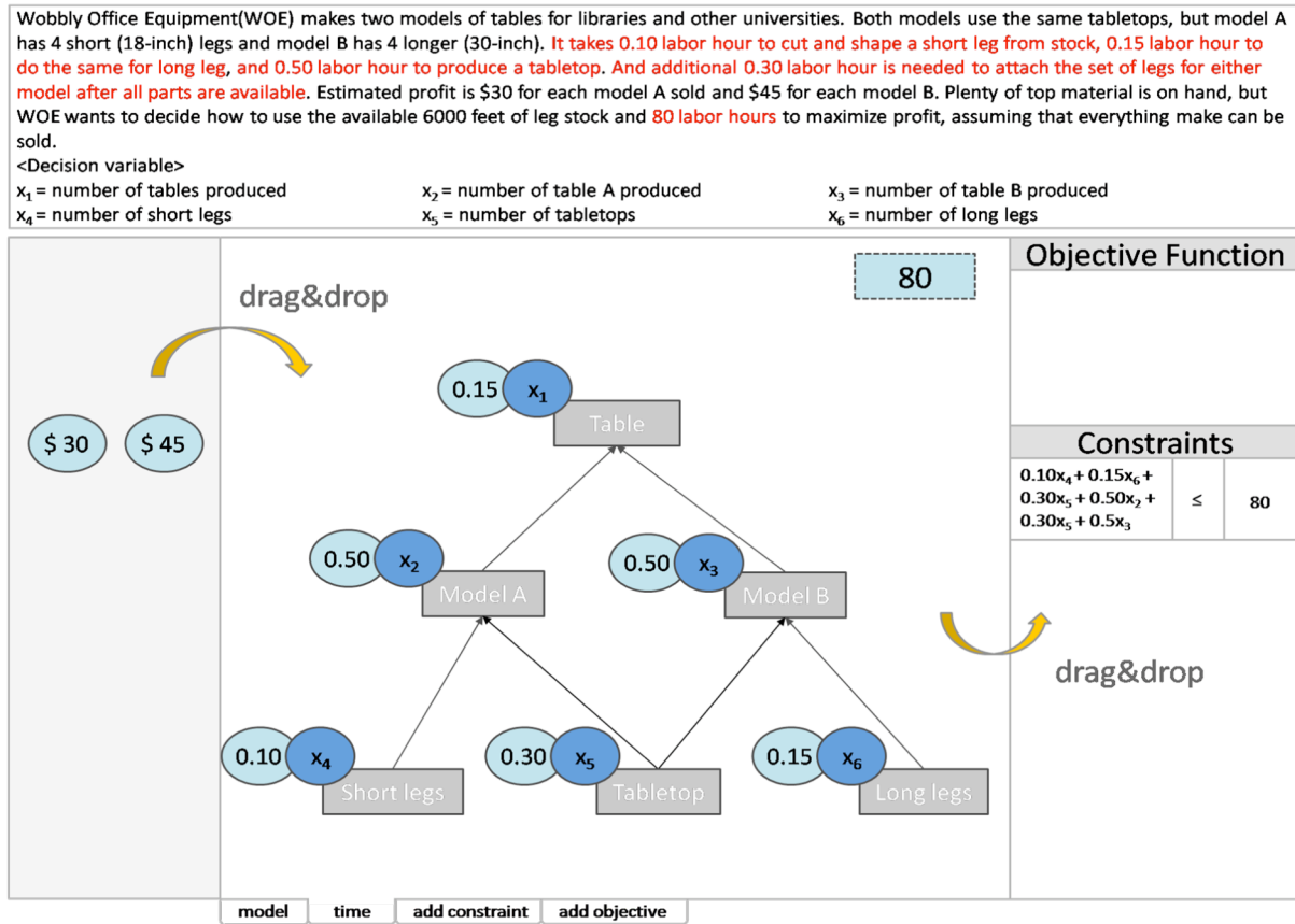
Figure 1. Screenshot of the visualization tool prototype
